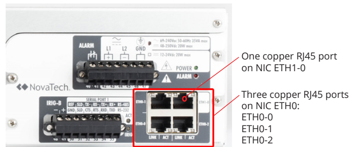
Figure 3 – Orion I/O with Ethernet Switch
